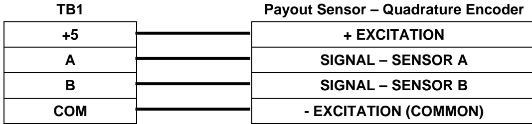
Figure 2.2 – Payout Sensor Hookup – 5VDC Quadrature Encoder
