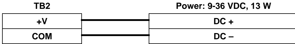
Figure 4.2 - Local Display Power Hookup
