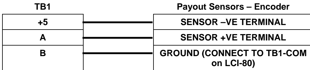
Figure 4.5 - Payout Sensor Hookup - Magnetic Pickup
