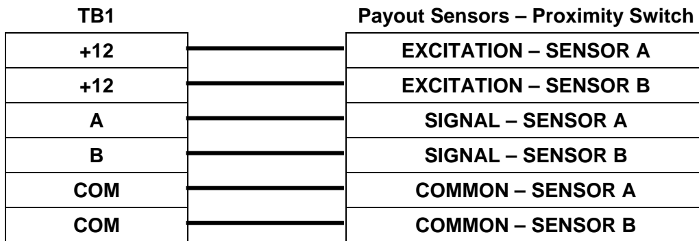
Figure 4.3 - Payout Sensor Hookup - 12V NPN/PNP switches
