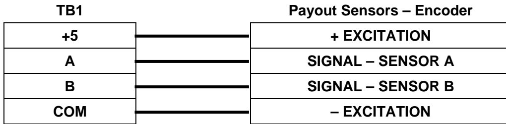
Figure 4.4 - Payout Sensor Hookup - TTL Encoder
