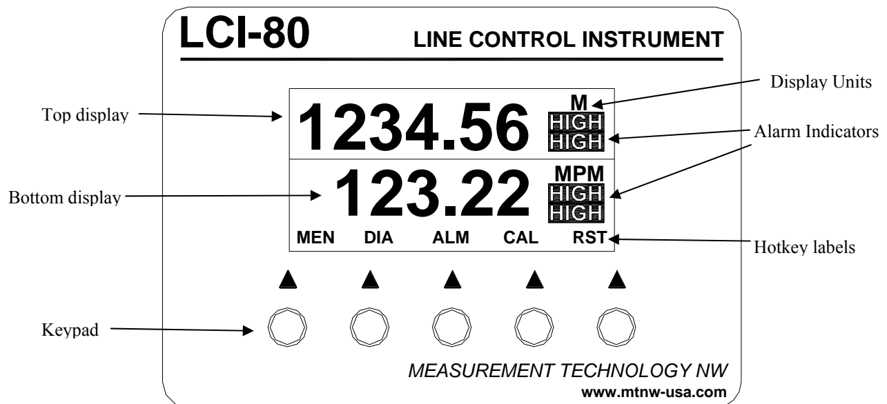
Figure 5.1 - LCI-80 Front Panel
