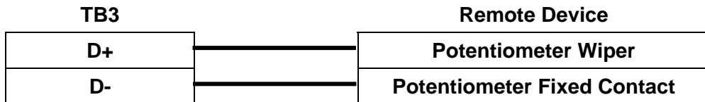
Figure 4.12 - Dimming Port Connection
