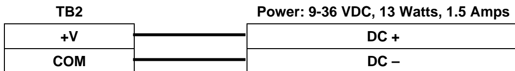
Figure 2.1 – Power Hookup – DC Power
