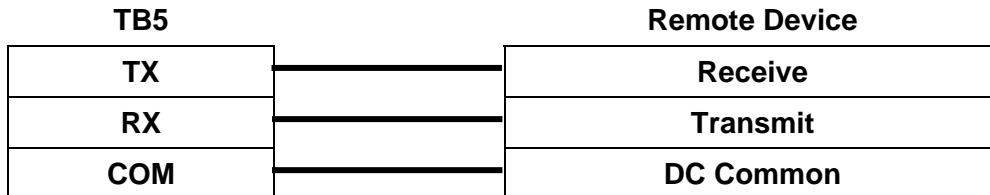
Figure 4.8 - RS-232 Serial Port Connection
