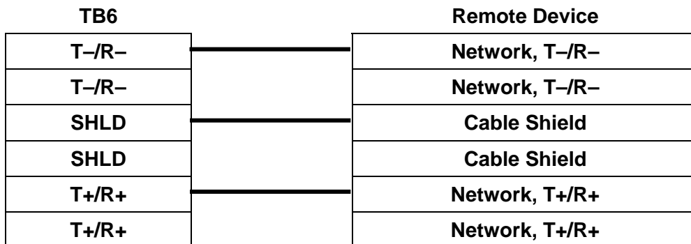
Figure 4.9 - RS-485 Serial Port Connection
