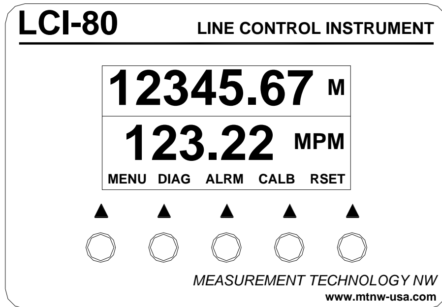
Figure 1.1 – LCI-80 Front Panel
