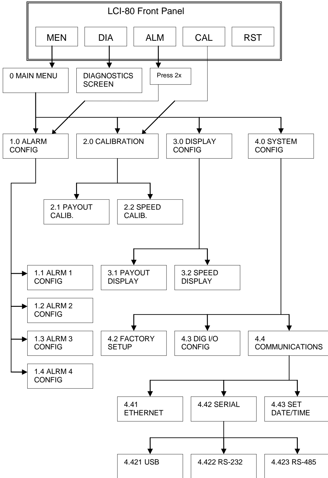
Figure 5.2 - LCI-80 Menu Tree
