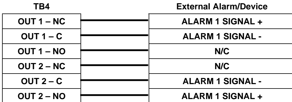
Figure 4.6 - Alarm Output Hookup
